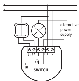
Fig.1 Circuit diagrams for Fibaro Switch.
